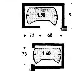
18 Wall cupboards for folding beds
